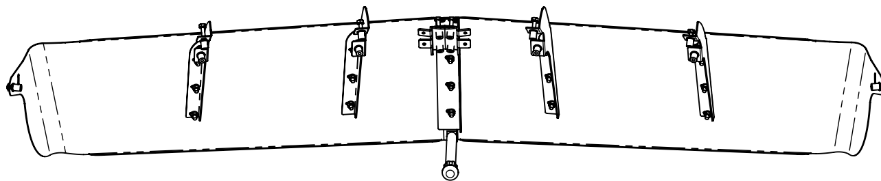
SUN VISOR ASSEMBLY BACK VIEW
